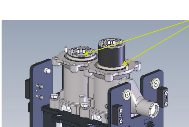
Fig. 5-4: Replacement of the composite piston seal
