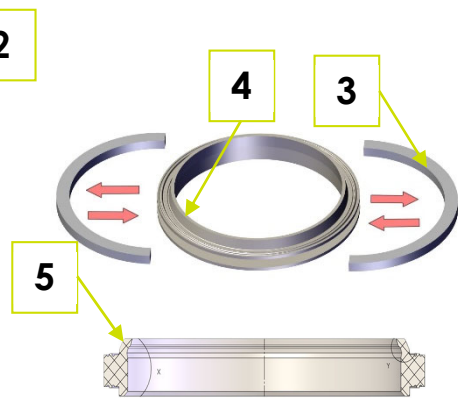
Fig. 5-6: Structure of the composite piston seal
