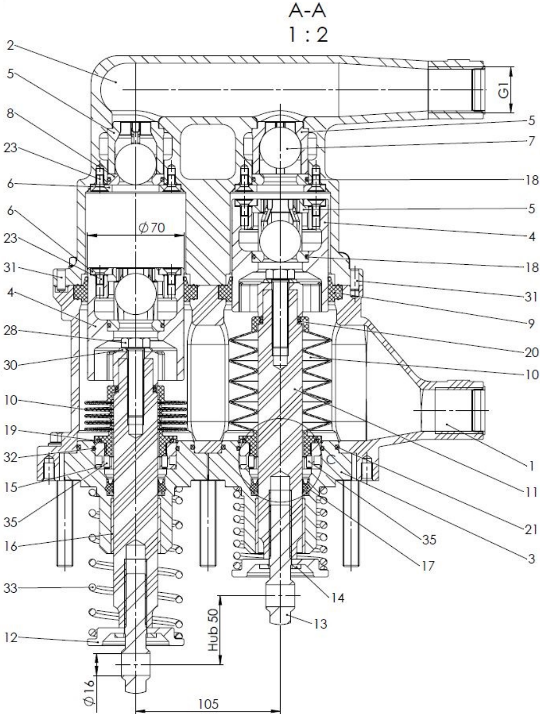
Fig. 8-1: Assembly drawing – pump unit
