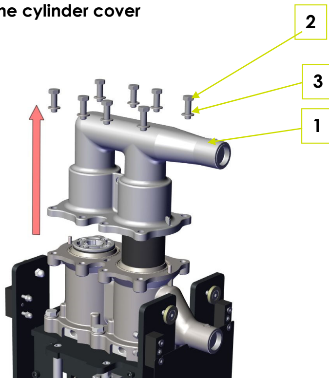
Fig. 5-1: Dismounting the cylinder cover
