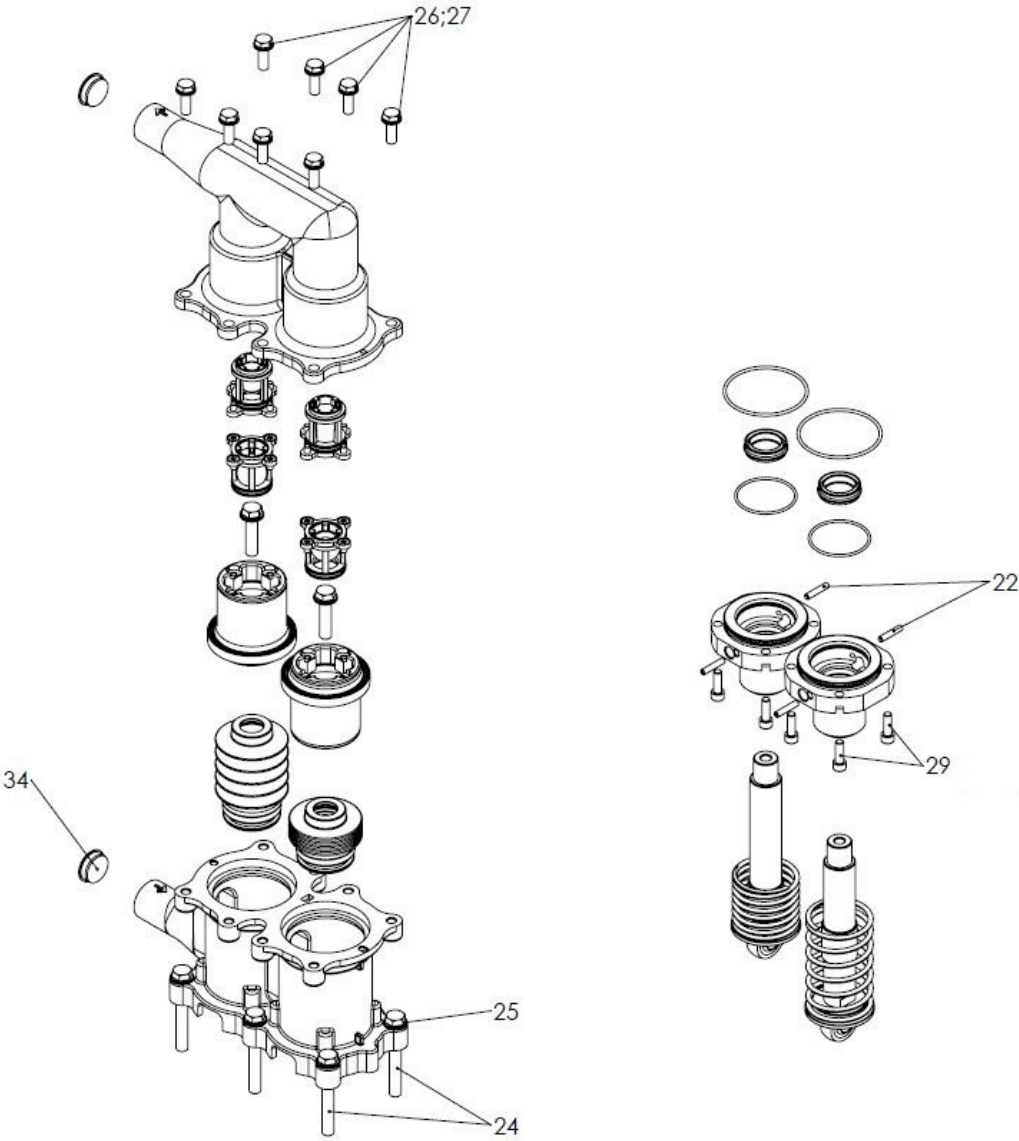
Fig. 8-2: Exploded-view drawing – pump unit
