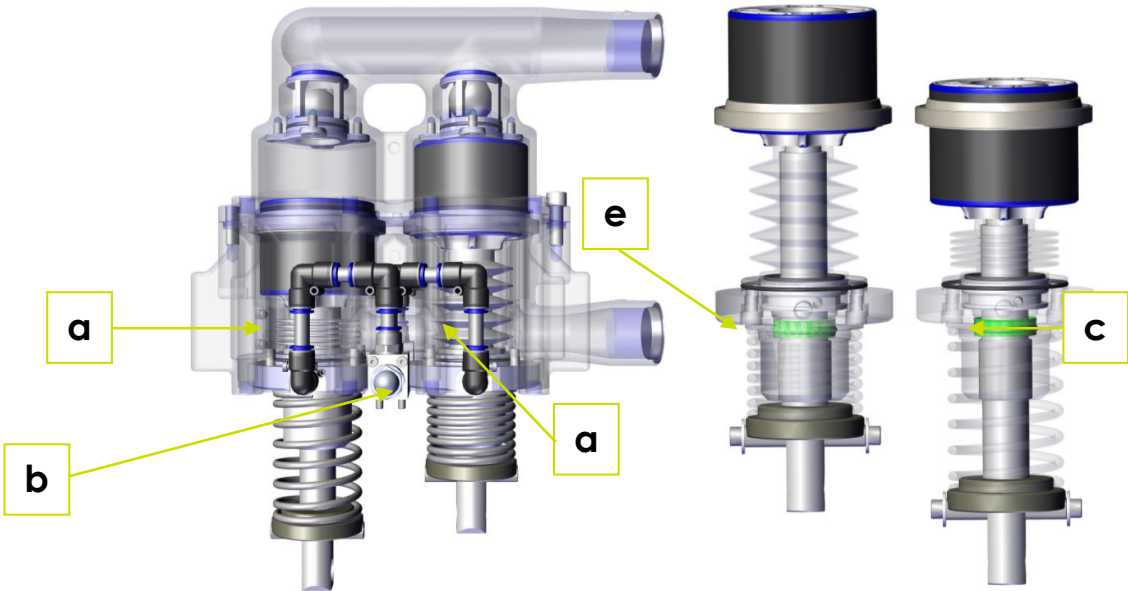
Figure 4-7 Seals
