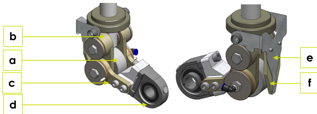
Figure 4-3 Double-joint rocker with lubricating rocker
