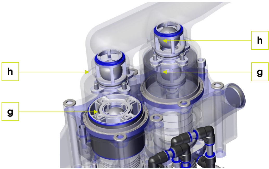
Figure 4-5 Pump head
