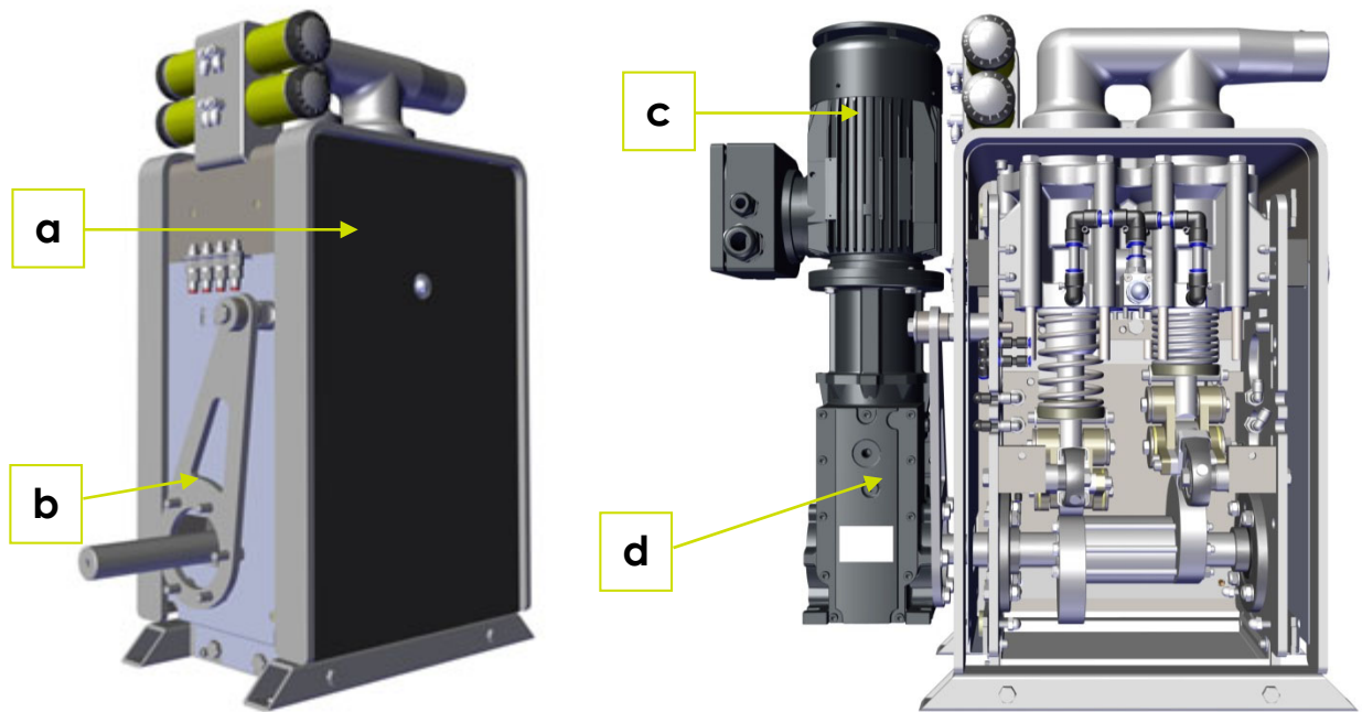
Fig. 5-1: Installation of motor and gearbox (example)
