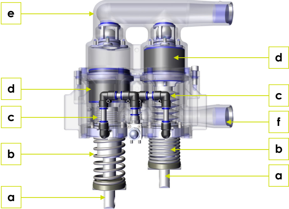
Figure 4-4 Pump head
