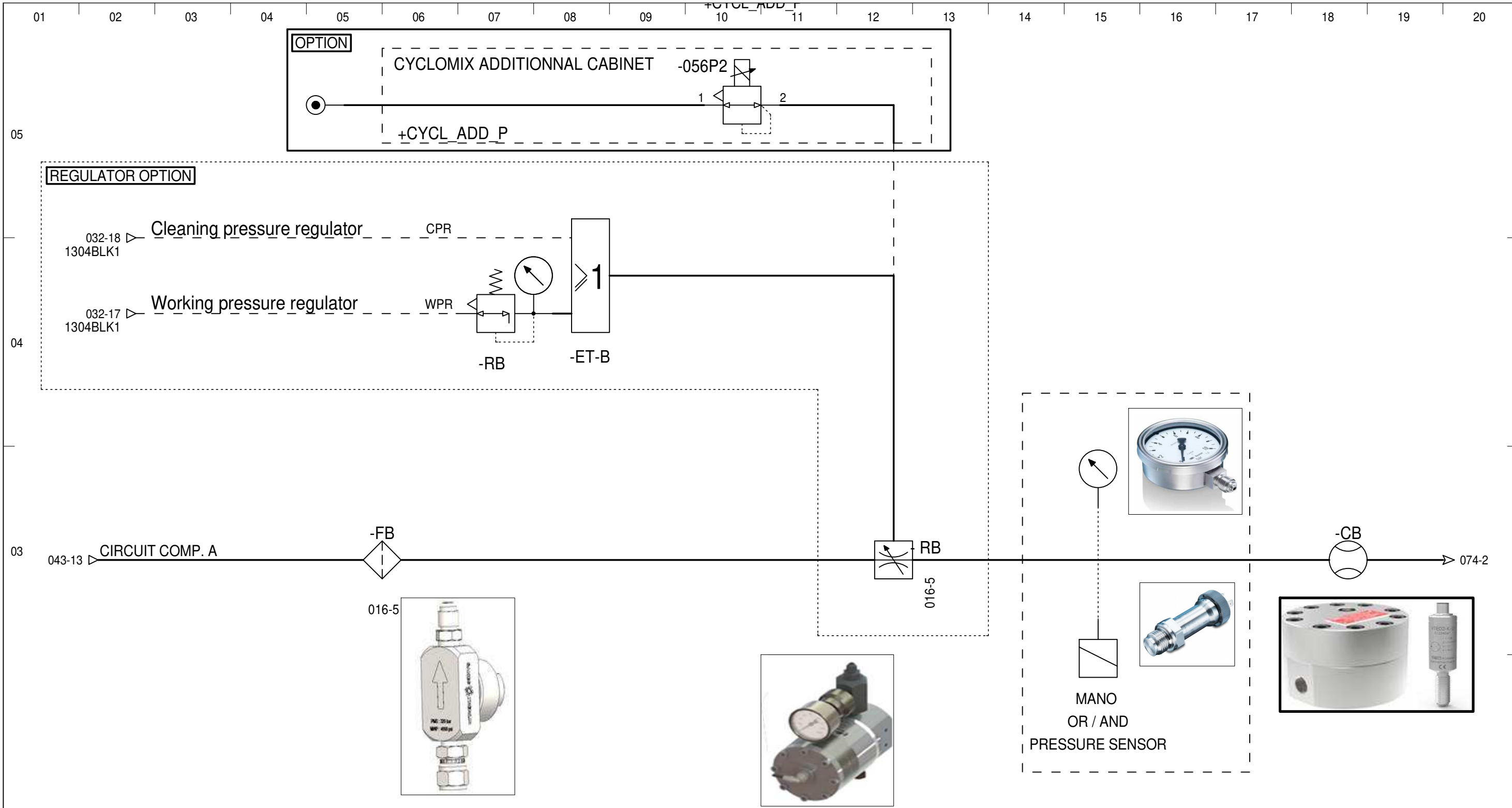
OPTION REGULATOR
